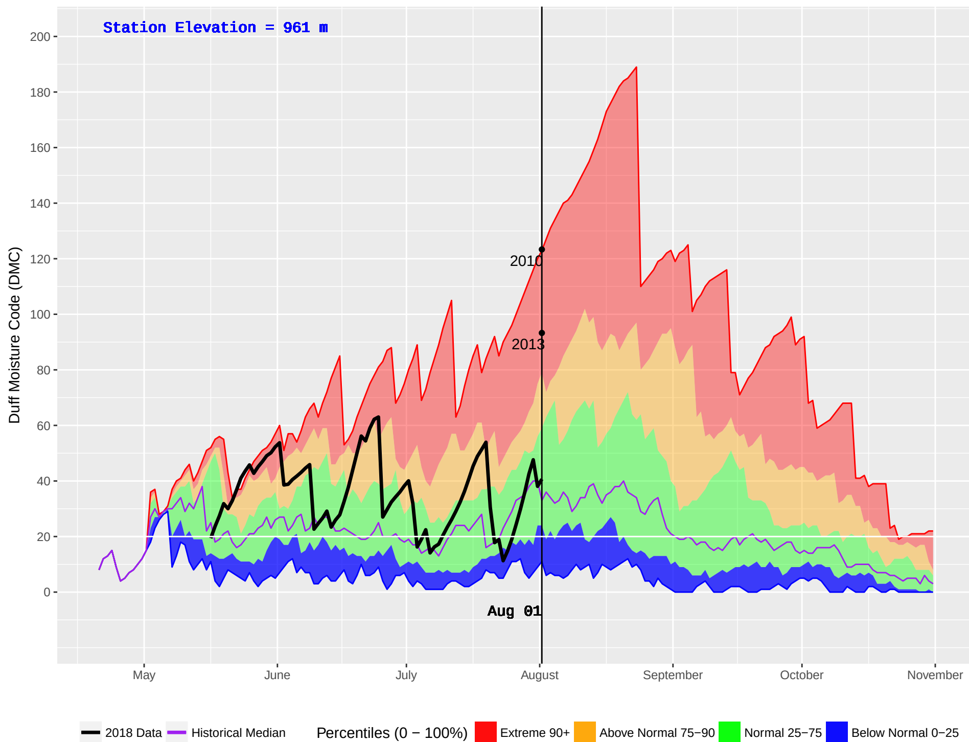
HOLY CROSS 2 (654) : Historical (1998–2016) and Current (2018) Daily Duff Moisture Code (DMC)
